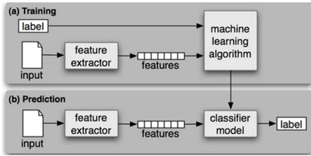
Fig. 1. Supervised classification [3].
