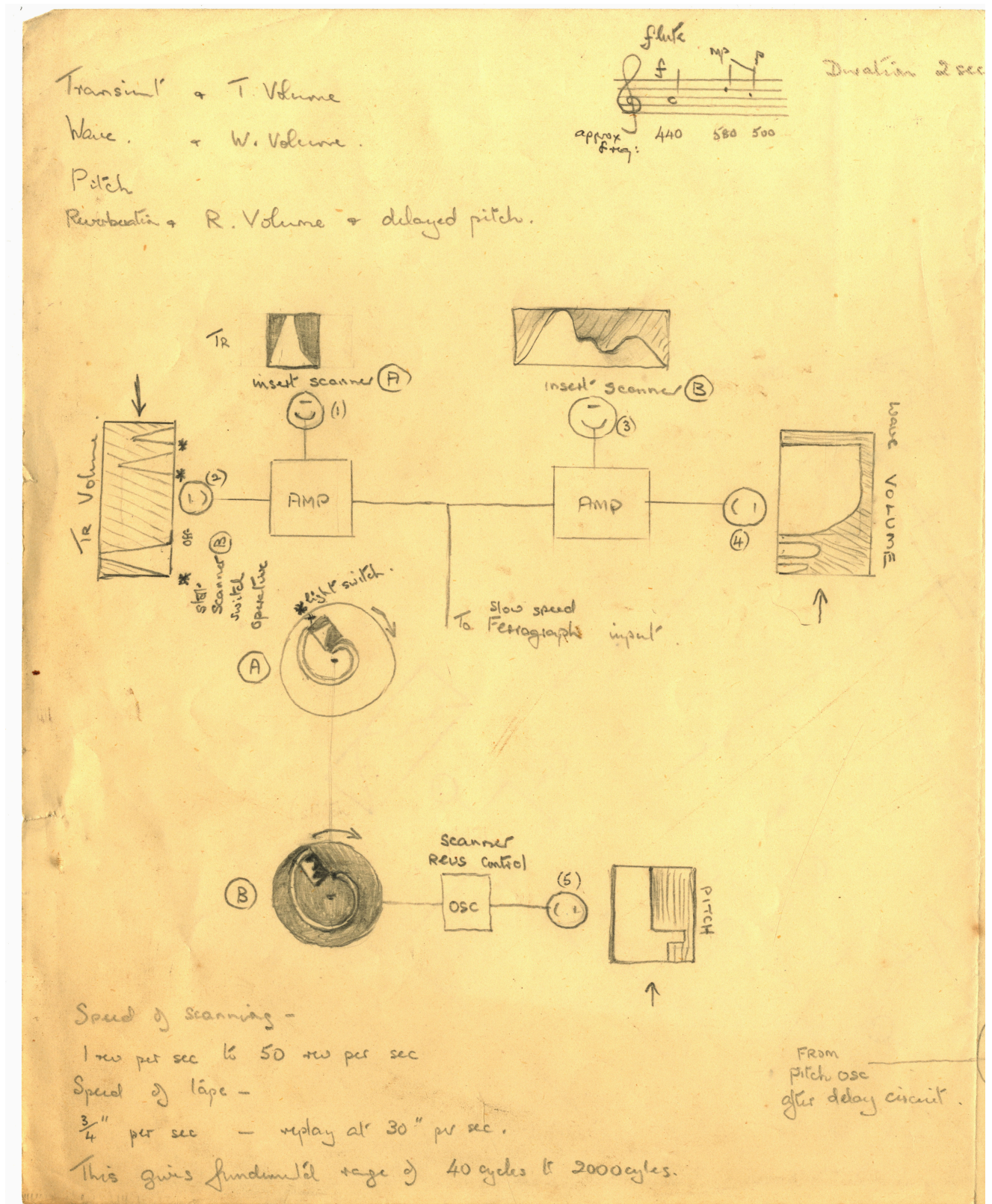
Fig. 12: Design by Daphne Oram, illustrating the overall system she envisaged for the production of music using drawn sound, circa 1957. Oram 2007, ORAM01/01/011
