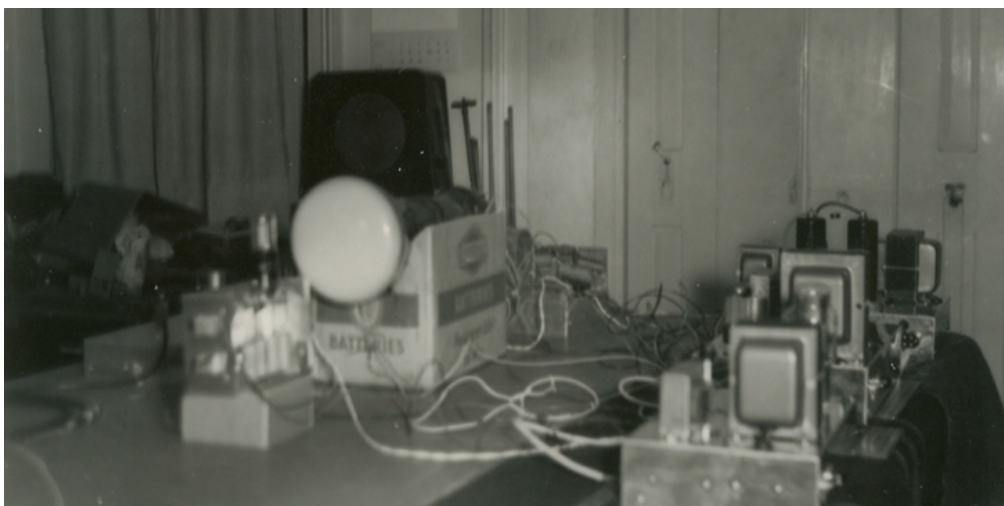
Fig. 16. Experimental Wave Scanner at Tower Folly, Early 1960s. Oram 2007, ORAM 07/04/053
