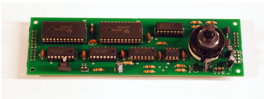
Fig. 37. Multiplexer circuit board for the graphic-oscillator section. February 2016
