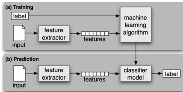
Fig. 1. Supervised classification [3].
