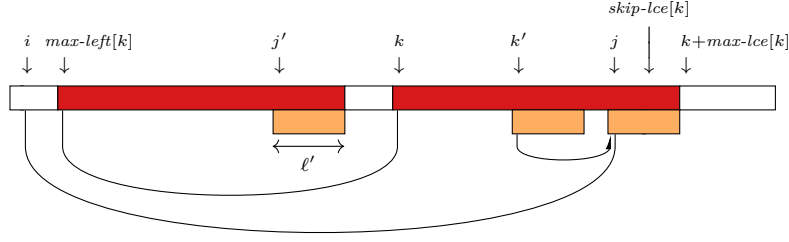
■ Figure 5 Supplementary drawing for Property 18.
