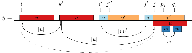
■ Figure 4 Supplementary drawing for the proof of Lemma 14. (Best viewed in colour.)
